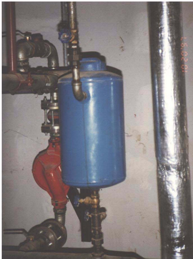
Pot feeder 16 liters made by Akiki Engineering
